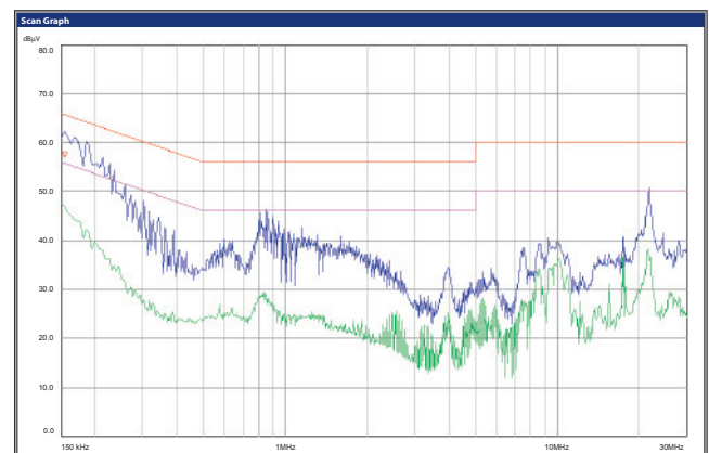
EMC characteristic
